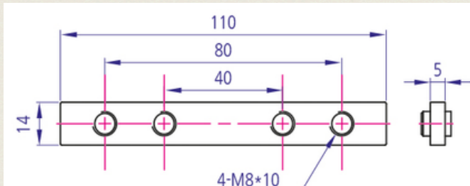
Inner Bracket P/N: ES-MLN-08 (40)
